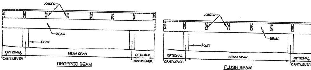
FIGURE R507.6 TYPICAL DECK BEAM SPANS
